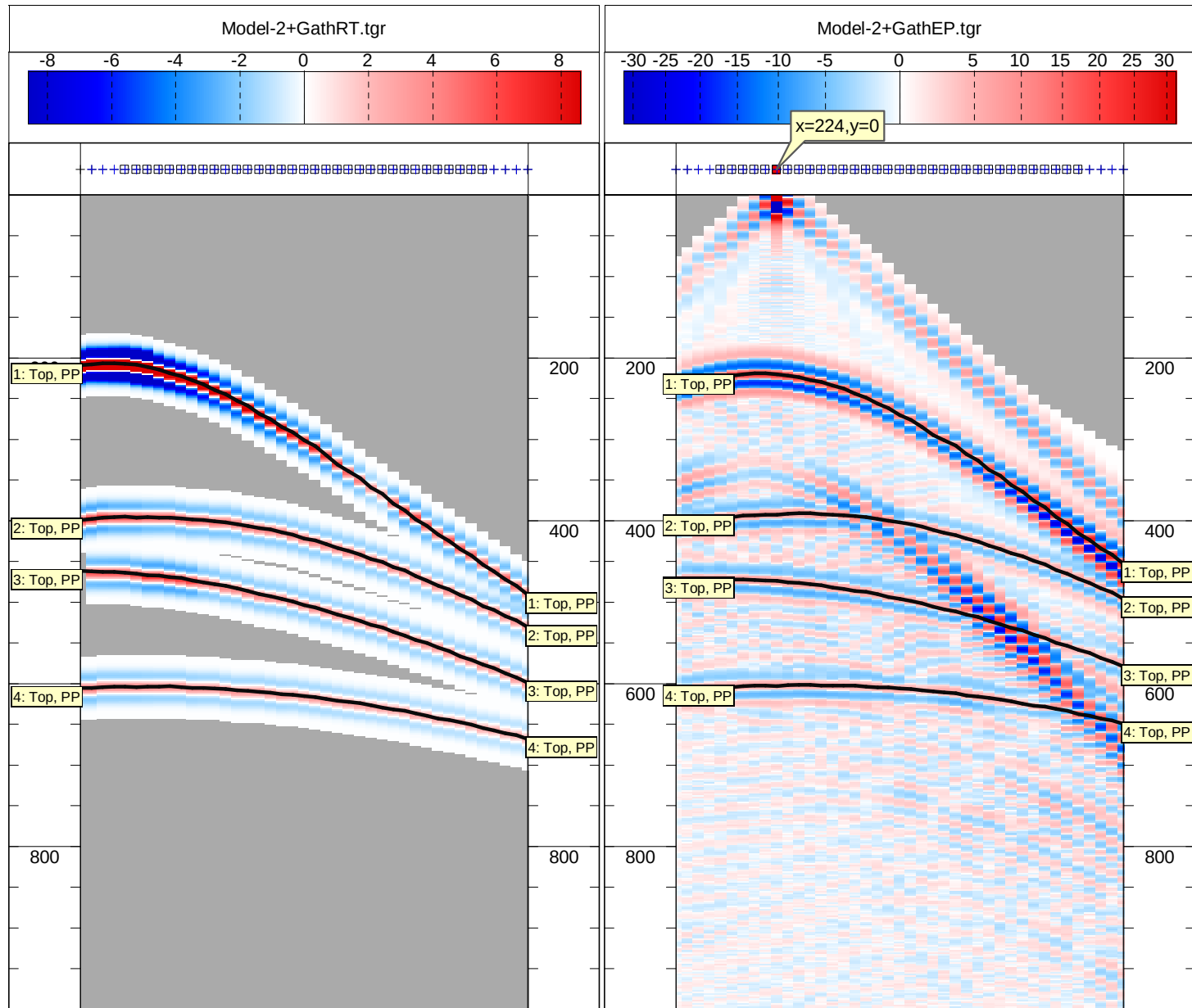
Ray Reflection Times on the Ray-Tracing Shotgather
