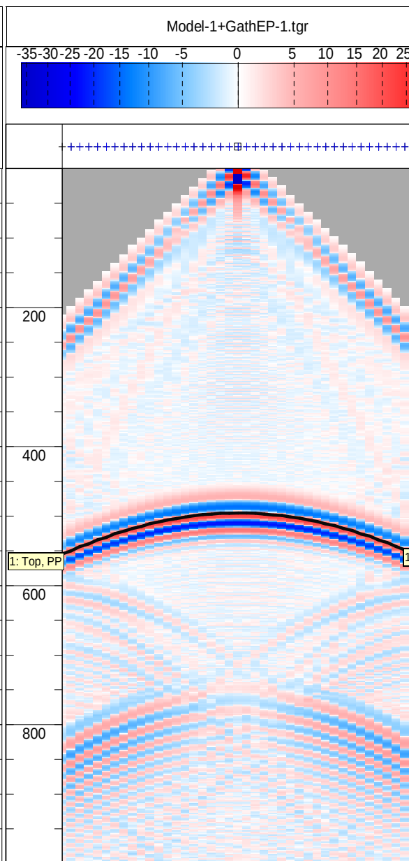
Ray Reflection Times on the Elastic finite-difference Shotgather
