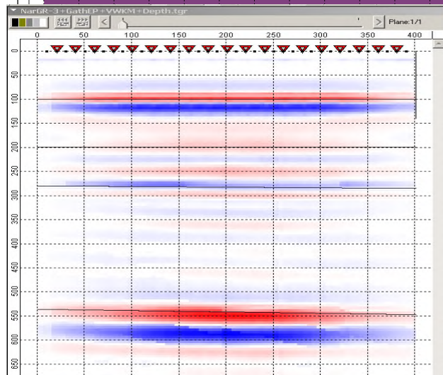
Migration using finite-difference shotgathers EP
