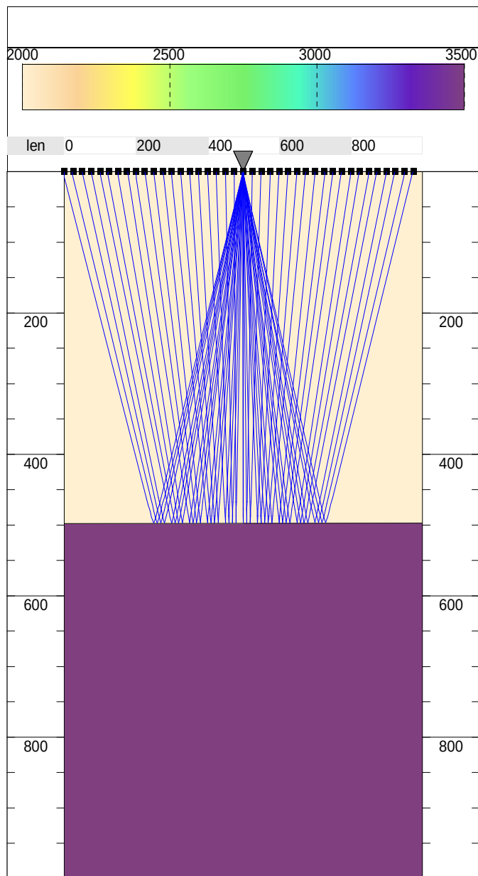
Ray Paths
