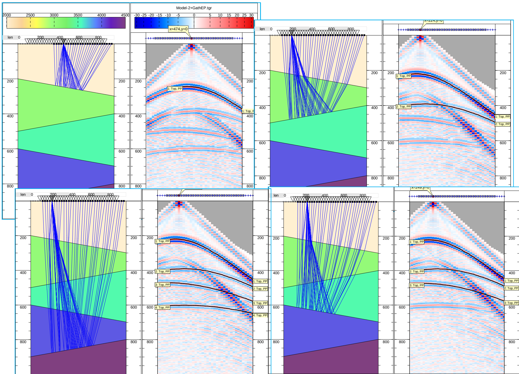
Ray Paths for different reflecting boundaries
