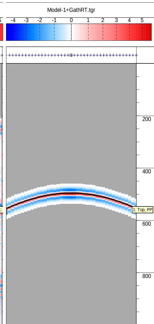
Ray Reflection Times on the Ray- Tracing Shotgather
